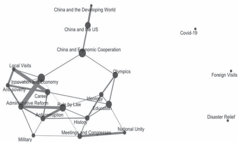
Figure 3. The network of correlated topics for a 20-topic Structural Topic Model. Node size is proportional to centrality and edge width is proportional to the strength of the correlation between topics.
